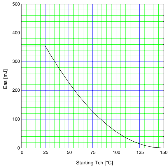
Maximum Avalanche energy vs. starting Tch E_{as} = f(\text{starting Tch}) : V_{cc} = 24V_{AV}, I_{AV} \leq 20A, \text{Non-Repetitive}
